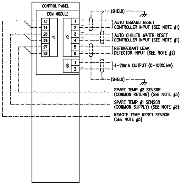
CONTROL PANEL OPTIONAL WIRING
