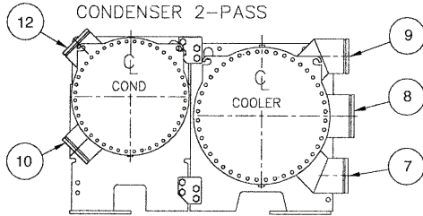
DISCHARGE END
