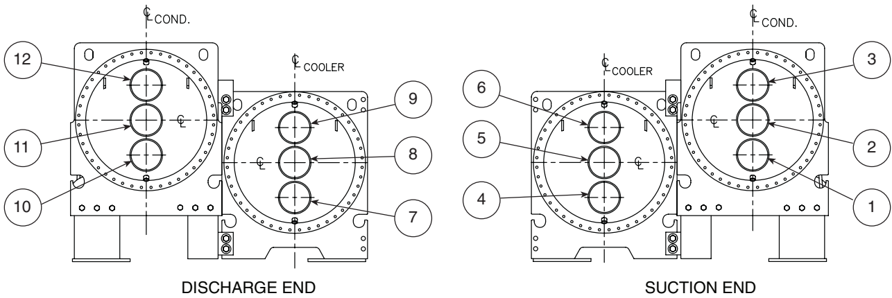
FRAMES 4 AND 5
