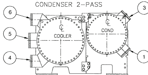
SUCTION END
