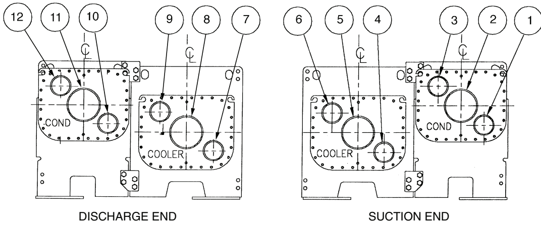
FRAME 3
