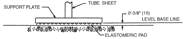
VIEW Y-Y
