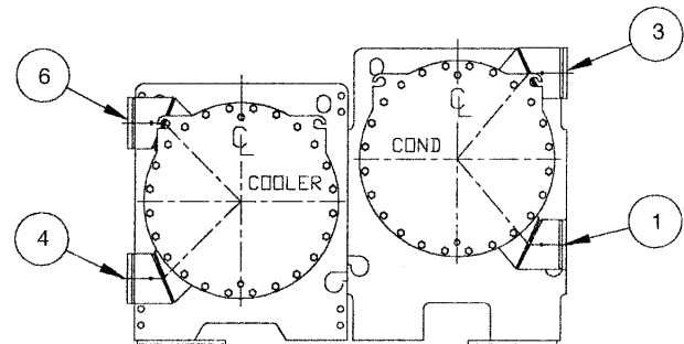
SUCTION END
