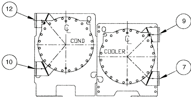
DISCHARGE END
